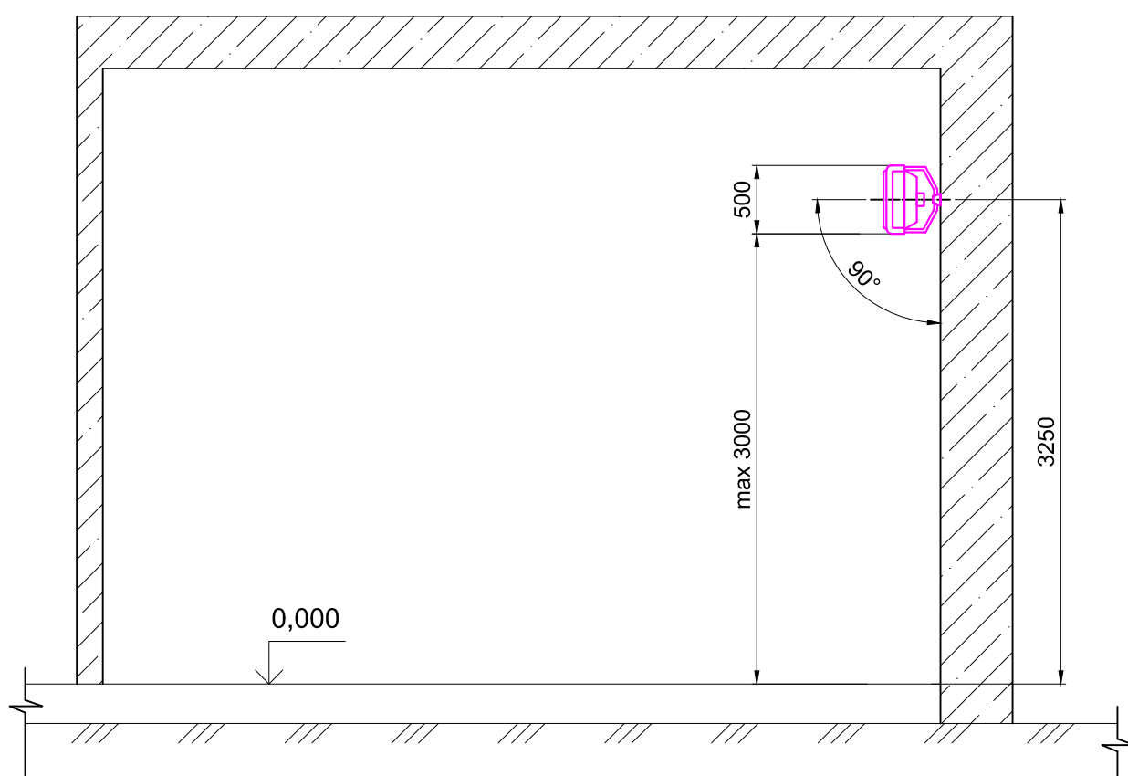
1 - 1 (1:50)
