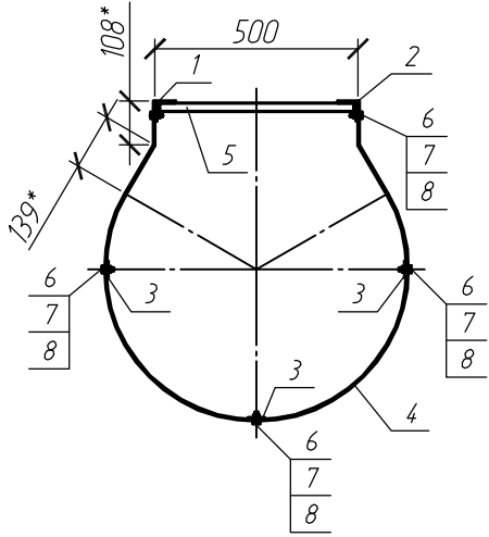
1-1 (1:20)
